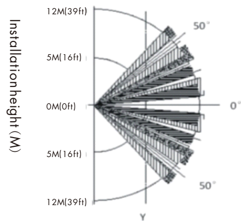
Wall installation detection range map
